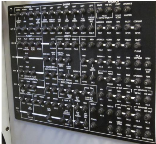
Image 20: Co-pilot Circuit Breaker Panel
