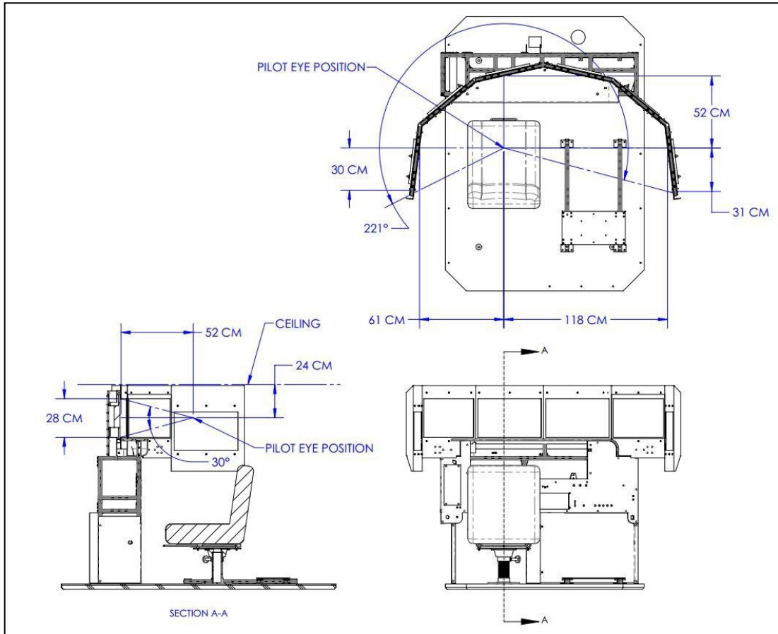
Image 32: Designated Eye Point Diagram
