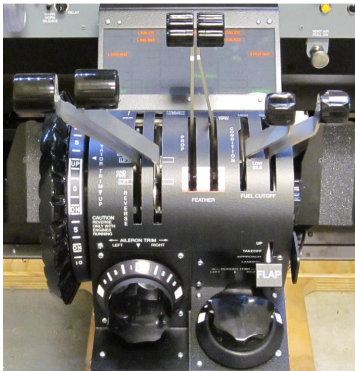
Image 16: Throttle Quadrant
